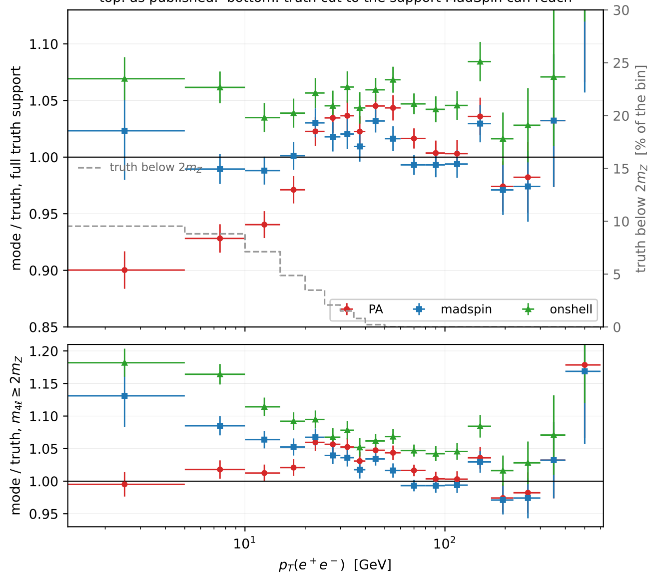
gg \rightarrow ZZ (loop induced) + MadSpin vs the off-shell truth top: as published. bottom: truth cut to the support MadSpin can reach
