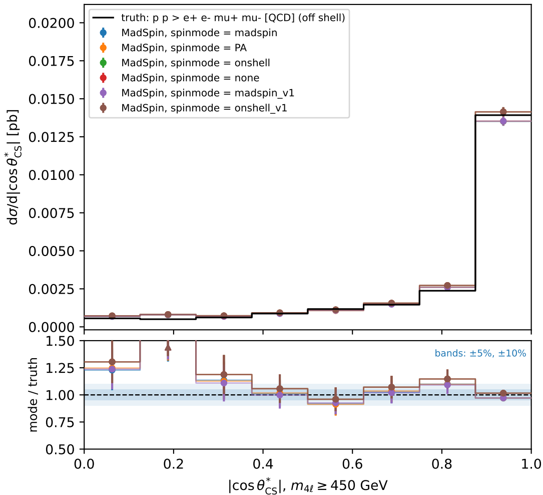
pp \rightarrow ZZ [QCD] (MC@NLO) \rightarrow e^+e^-\mu^+\mu^- , 13 TeV — shape-study observables
