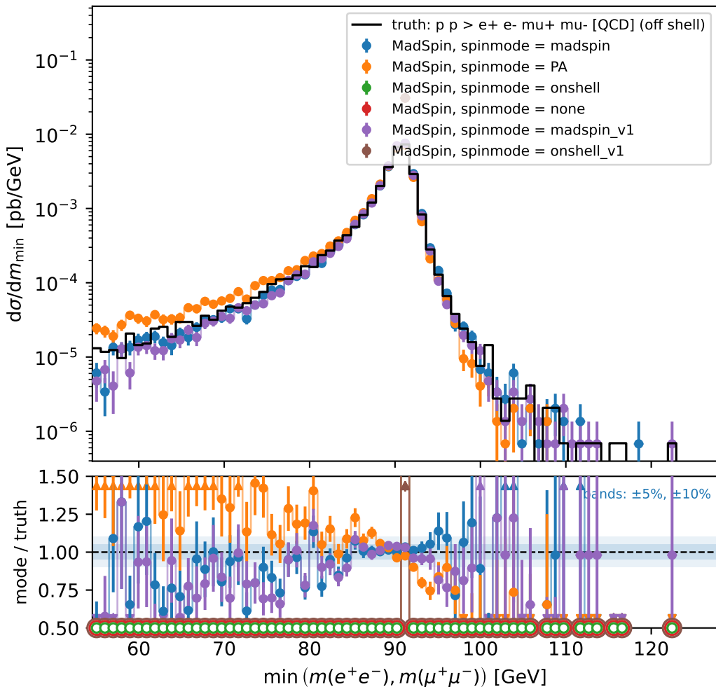
pp \rightarrow ZZ [QCD] (MC@NLO) \rightarrow e^+e^-\mu^+\mu^- , 13 TeV — shape-study observables
