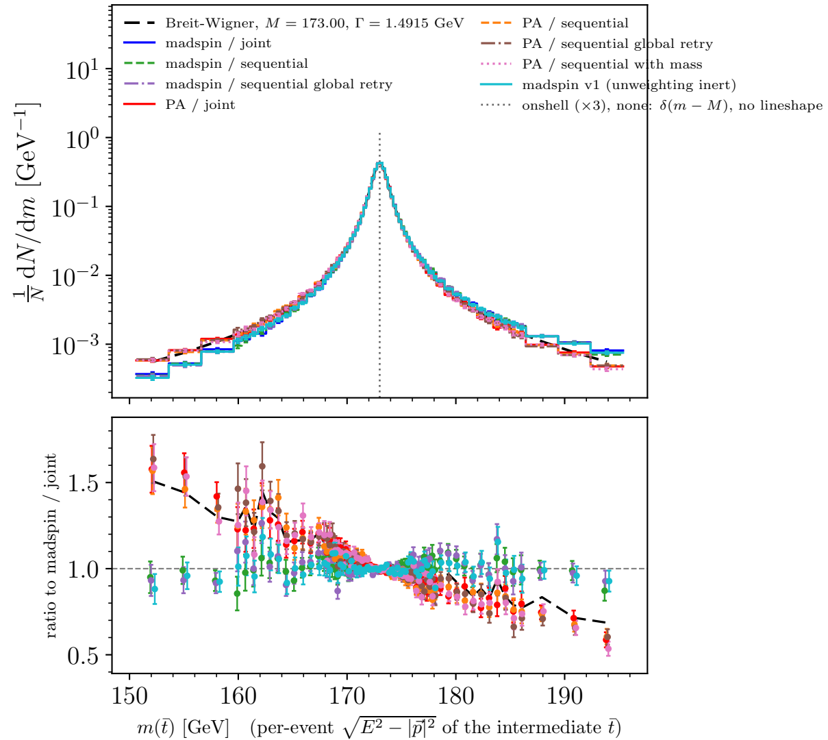
MadSpin m(\bar{t}) lineshape: every distinct spinmode / unweighting cell
