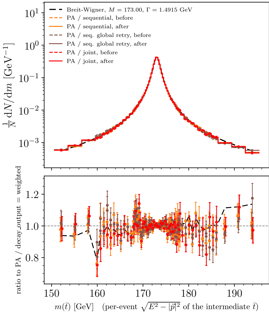
PA: the per-event mass bound, before and after
