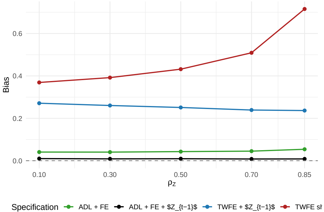
Figure 2: Dual-role simulation: ADL + FE with lagged state variables dominates static alternatives. In the main design, ADL + FE + Z_{t-1} keeps bias near zero across the full range of collider persistence, while TWFE remains biased even when it includes Z_{t-1} .
