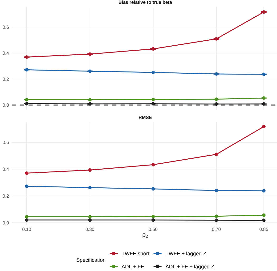
Figure 4: Dual-role DGP: bias relative to the true contemporaneous treatment effect and RMSE across collider persistence. The DGP has Z_{t-1} as a confounder and Z_t as a contemporaneous collider; the estimand is \beta = 1 . The displayed subset sets \sigma_{\alpha_Z} = 0.5 , with N = 100 , T = 30 , a burn-in of 100 periods, and 500 Monte Carlo replications per scenario. Models are TWFE short, TWFE plus Z_{t-1} , ADL+FE, and ADL+FE plus Z_{t-1} ; FE models include unit and time effects. Error bars are 95% Monte Carlo uncertainty intervals for simulated mean bias, not estimator confidence intervals.
