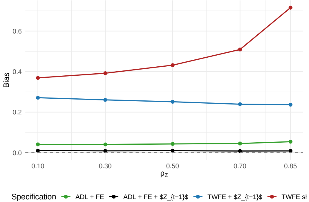
Figure 2: Dual-role simulation: ADL + FE with lagged state variables dominates static alternatives. In the main design, ADL + FE + Z_{t-1} keeps bias near zero across the full range of collider persistence, while TWFE remains biased even when it includes Z_{t-1} .
