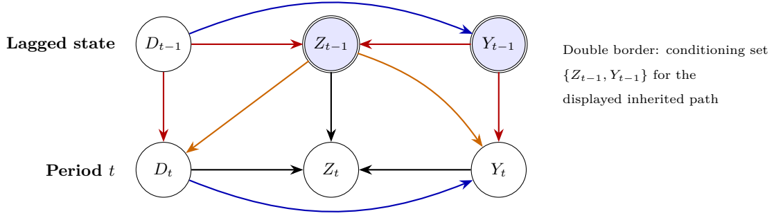
Figure 3: Dynamic dual-role DAG. Orange arrows form the lagged-confounding fork; red arrows trace the inherited collider path. Conditioning on Z_{t-1} blocks the former but opens the latter. Conditioning additionally on Y_{t-1} blocks that inherited path, subject to the displayed DAG and the paper’s timing and identification conditions.
