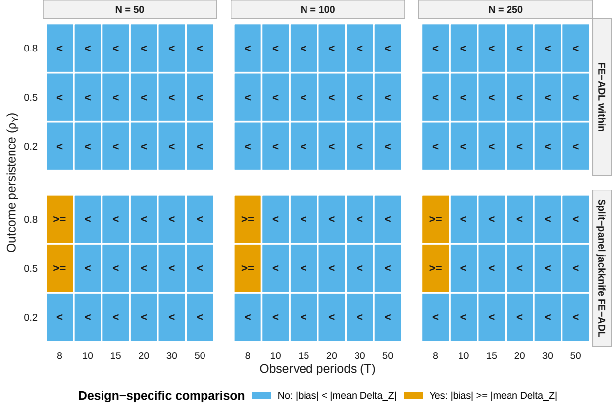
Figure 5: Finite- T phase map for the principal dual-role grid. Each tile reports the design-specific comparison |\text{Monte Carlo bias}| \geq |\text{mean}(\Delta_Z)| for the long FE-ADL within estimator or its split-panel jackknife correction. Columns vary N , the horizontal axis varies T , and the vertical axis varies outcome persistence \rho_Y ; each cell contains 500 Monte Carlo replications with \beta_{\text{CET}} = 1 . Symbols redundantly encode the color categories. This diagnostic comparison does not define an acceptable- T threshold. Arellano-Bond, the stress grid, and full provenance are reported in the Task 13 report/online appendix.
