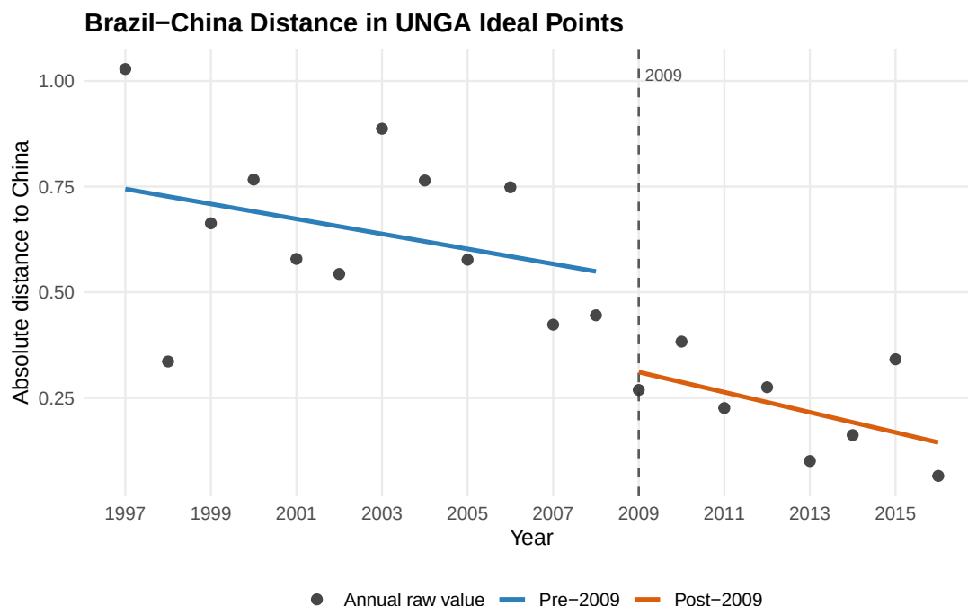
Figure 1. Descriptive only. Lines are separate OLS fits before 2009 and from 2009 onward. The dashed line marks China's rank reversal in Brazil's trade hierarchy.
