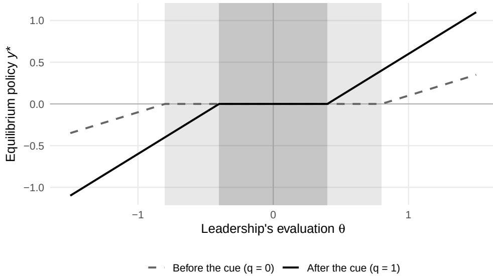
Figure 1: Equilibrium policy response y^*(q) as a function of the leadership's evaluation \theta , before ( q = 0 ) and after ( q = 1 ) the public cue. Illustrative values: s(0) = 0.5 , s(1) = 1 , c_L = 0.4 , and K(q) > c_B in both states. In the dark band, neither state produces a response; in the light bands, a response occurs only after the cue.
