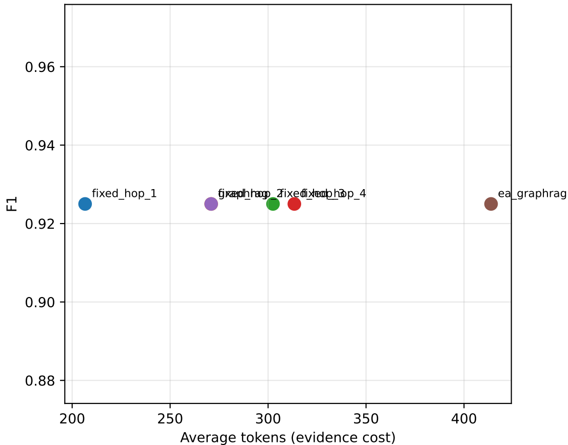
E3: Accuracy vs Evidence Cost
