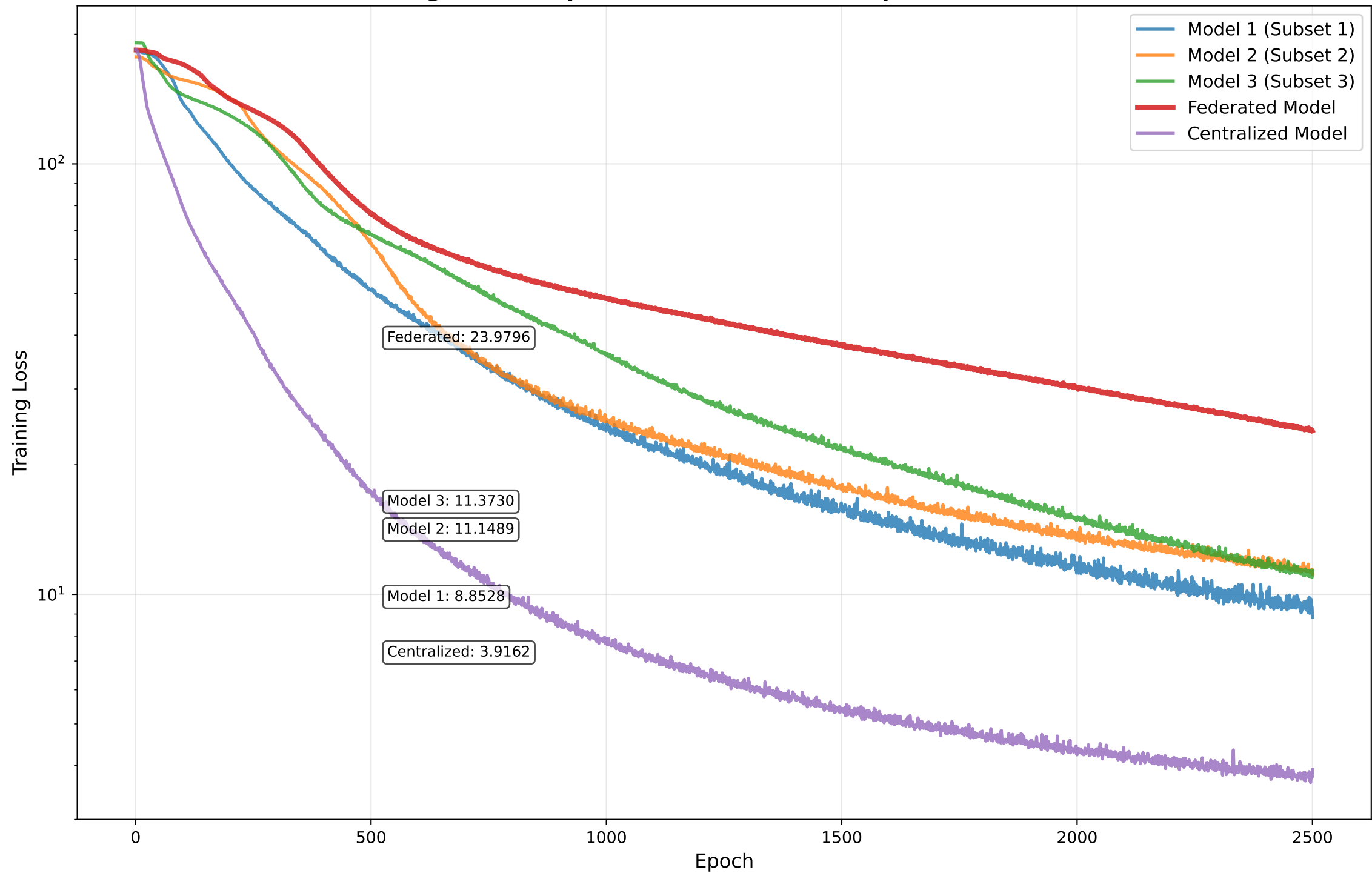
Training Loss vs Epoch - All Scenarios Comparison (FedProx)
