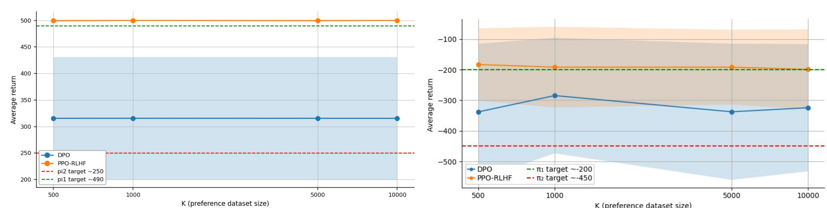
Figure 4. Average true episode return at the end of fine-tuning as a function of preference dataset size K, on CartPole-v1 (left) and Pendulum-v1 (right). Orange: PPO-RLHF, blue: DPO. Shaded regions indicate standard deviation across seeds. Dashed lines mark the \pi_1 (expert) and \pi_2 (mediocre) checkpoint returns for reference.
