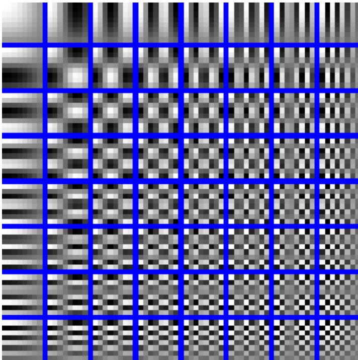
DCT Basis Function for N=8
