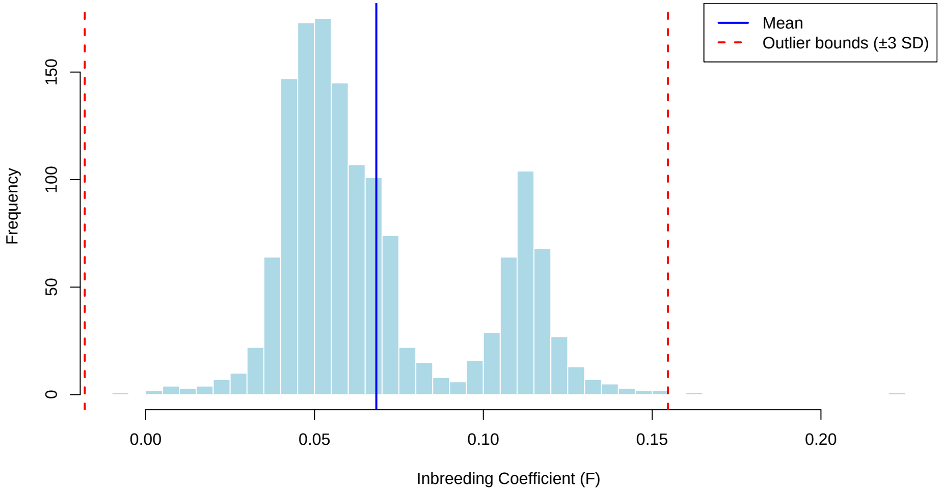
Distribution of Heterozygosity (F statistic)
