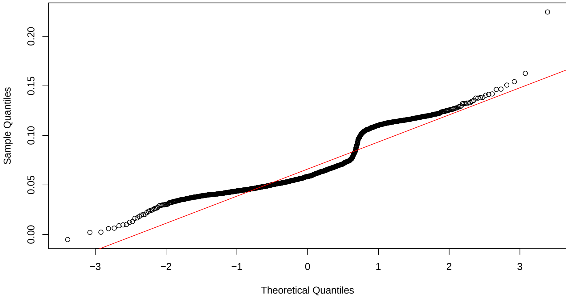
Q-Q Plot: Heterozygosity
