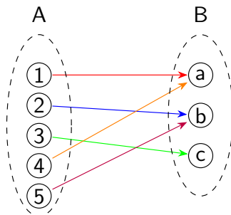
Surjective
