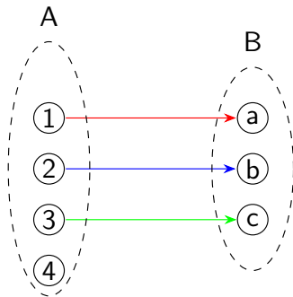
Injective
