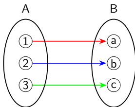
Bijection
