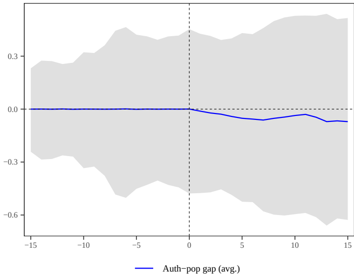
Pooled SCM: strict
