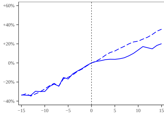
\lambda=0.1 (N=6)
