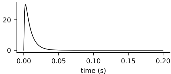
biexp(amp=30, tau_rise=1ms, tau_decay=8ms)
