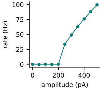
f-I curve of the model
