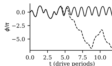
Figure 2: Two driven, damped pendulums released from angles that differ by one part in a thousand. For five drive cycles you cannot tell them apart; then one flips over the top and they never agree again. Week 14.
