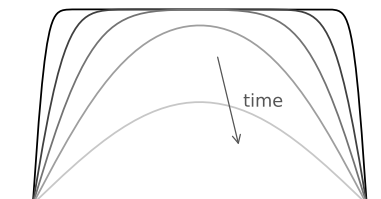
Figure 2: A uniformly hot bar with its ends held cold, relaxing toward equilibrium. The sharp corners disappear almost instantly — by week 15 you’ll know why.
