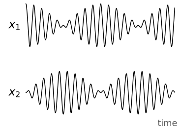
Figure 1: Two coupled oscillators trading energy back and forth. By week 9 you will be able to predict this motion exactly, and in week 15 it becomes the wave equation.
