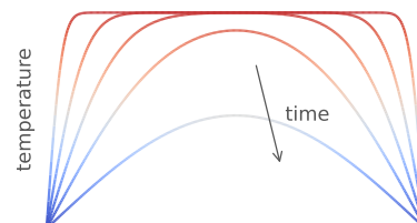
Figure 2: A uniformly hot bar with its ends held cold, relaxing toward equilibrium; color shows temperature. The sharp corners disappear almost instantly — by week 15 you’ll know why.
