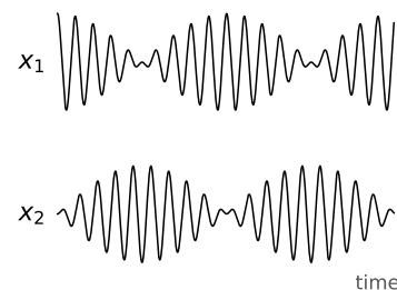
Figure 1: Two coupled oscillators trading energy back and forth. By week 9 you will be able to predict this motion exactly, and in week 15 it becomes the wave equation.
