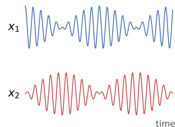
Figure 1: The displacements of two coupled oscillators as they trade energy back and forth: when one swings big, the other swings small. By week 9 you will be able to predict this motion exactly, and in week 15 it becomes the wave equation.
