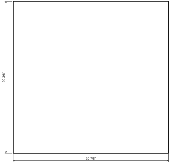
Drawer 1.2 bottom 6 mm plywood (backs) · T 1/4" · 20 7/8" x 20 3/8"
