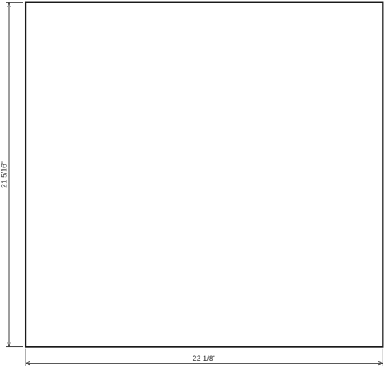
Shelf 1.1.1 18 mm plywood · T 11/16" · 22 1/8" x 21 5/16" → Grain along length
