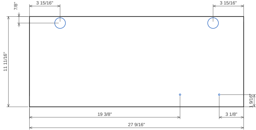
Door 1.1 right 18 mm MDF (paint-grade fronts) · T 11/16" · 27 9/16" x 11 11/16" No grain
