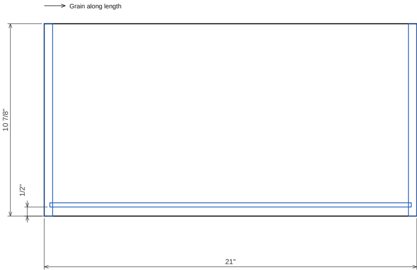
Drawer 1.3 right side 12 mm Baltic birch 4×8 (drawer boxes) · T 1/2" · 21" x 10 7/8" → Grain along length
