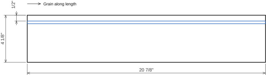
Drawer 1.1 box front 12 mm Baltic birch 4×8 (drawer boxes) · T 1/2" · 20 7/8" x 4 1/8"
