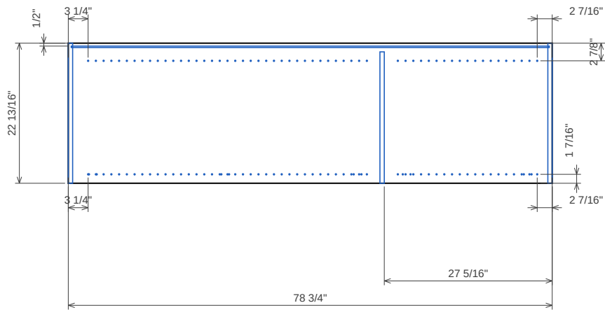
Right side 18 mm plywood · T 11/16" · 78 3/4" x 22 13/16" → Grain along length
