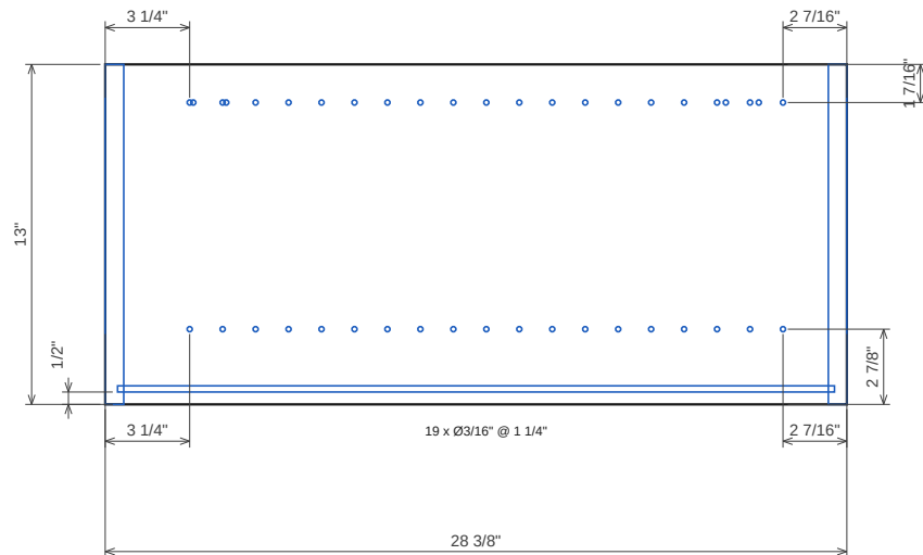
Left side 18 mm plywood · T 11/16" · 28 3/8" x 13" → Grain along length
