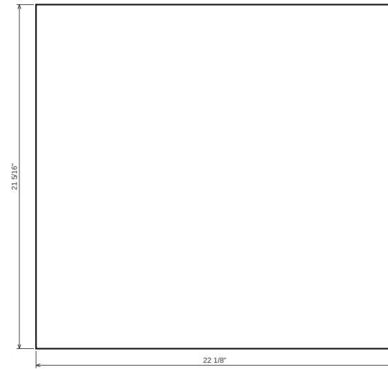
Shelf 1.2.3 18 mm plywood · T 11/16" · 22 1/8" x 21 5/16" → Grain along length
