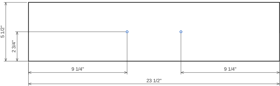
Drawer front 1.1 18 mm MDF (paint-grade fronts) · T 11/16" · 23 1/2" x 5 1/2" No grain
