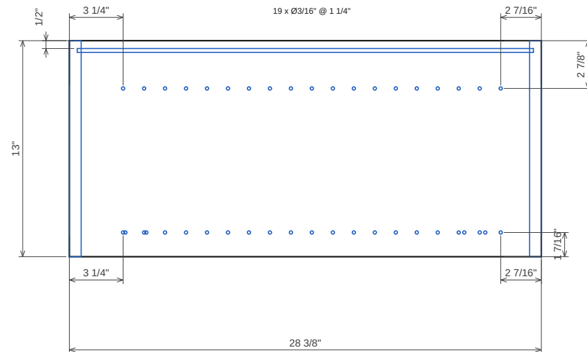
Right side 18 mm plywood · T 11/16" · 28 3/8" x 13" → Grain along length
