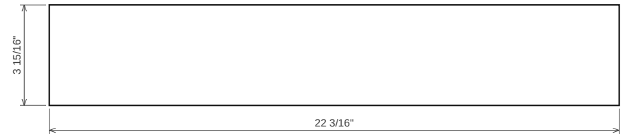
Bottom rear nailer 18 mm plywood · T 11/16" · 22 3/16" x 3 15/16" → Grain along length
