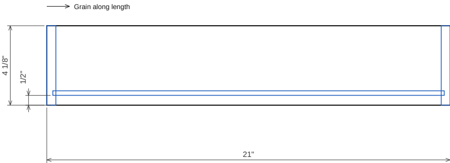
Drawer 1.1 right side 12 mm Baltic birch 4×8 (drawer boxes) · T 1/2" · 21" x 4 1/8"
