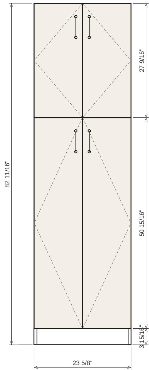
Tall pantry - front elevation
