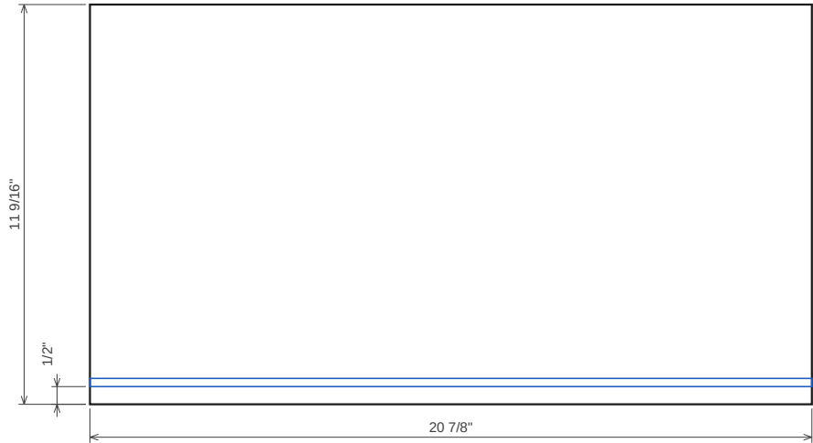
Drawer 1.2 box back 12 mm Baltic birch 4×8 (drawer boxes) · T 1/2" · 20 7/8" x 11 9/16"
