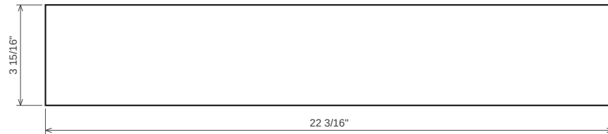
Top rear nailer 18 mm plywood · T 11/16" · 22 3/16" x 3 15/16" → Grain along length
