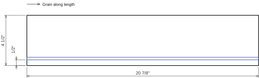
Drawer 1.1 box back 12 mm Baltic birch 4×8 (drawer boxes) · T 1/2" · 20 7/8" x 4 1/2"
