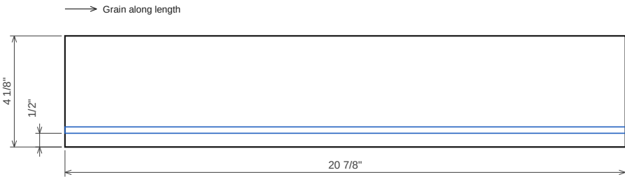
Drawer 1.1 box back 12 mm Baltic birch 4×8 (drawer boxes) · T 1/2" · 20 7/8" x 4 1/8"
