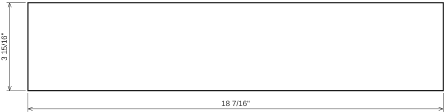
Kick sleeper 1 18 mm plywood · T 11/16" · 18 7/16" x 3 15/16" → Grain along length
