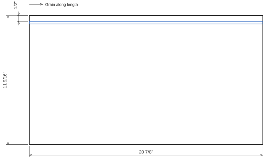
Drawer 1.2 box front 12 mm Baltic birch 4×8 (drawer boxes) · T 1/2" · 20 7/8" x 11 9/16"
