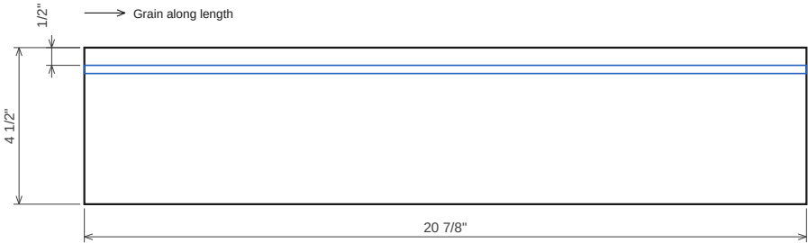
Drawer 1.1 box front 12 mm Baltic birch 4×8 (drawer boxes) · T 1/2" · 20 7/8" x 4 1/2"
