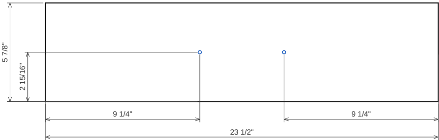
Drawer front 1.1 18 mm MDF (paint-grade fronts) · T 11/16" · 23 1/2" x 5 7/8" No grain
