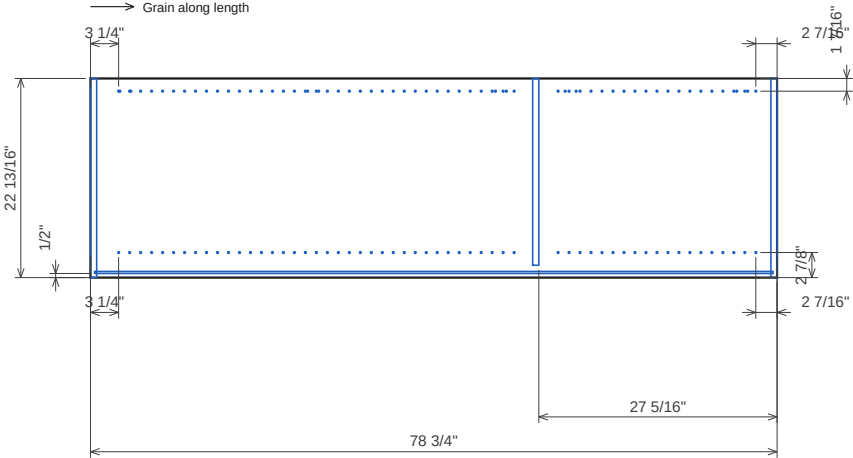
Left side 18 mm plywood · T 11/16" · 78 3/4" x 22 13/16" → Grain along length
