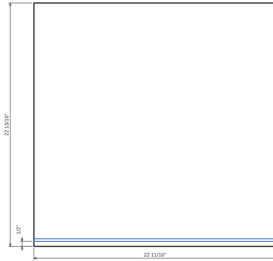
Top 18 mm plywood · T 11/16" · 22 11/16" x 22 13/16" → Grain along length
