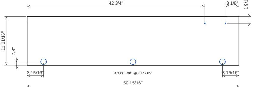
Door 1.2 left 18 mm MDF (paint-grade fronts) · T 11/16" · 50 15/16" x 11 11/16" No grain
