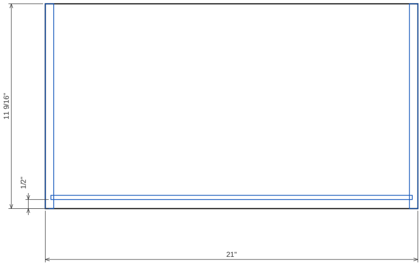
Drawer 1.2 right side 12 mm Baltic birch 4×8 (drawer boxes) · T 1/2" · 21" x 11 9/16" → Grain along length
