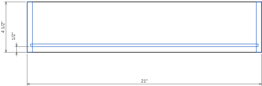
Drawer 1.1 right side 12 mm Baltic birch 4×8 (drawer boxes) · T 1/2" · 21" x 4 1/2" → Grain along length
