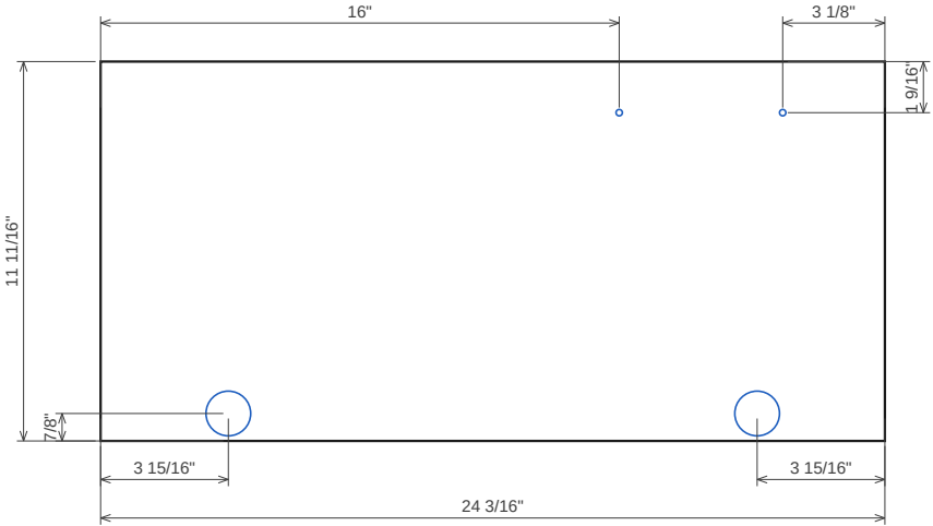
Door 1.2 left 18 mm MDF (paint-grade fronts) · T 11/16" · 24 3/16" x 11 11/16" No grain
