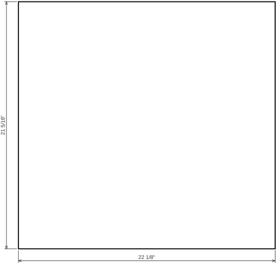
Shelf 1.2.1 18 mm plywood · T 11/16" · 22 1/8" x 21 5/16" → Grain along length
