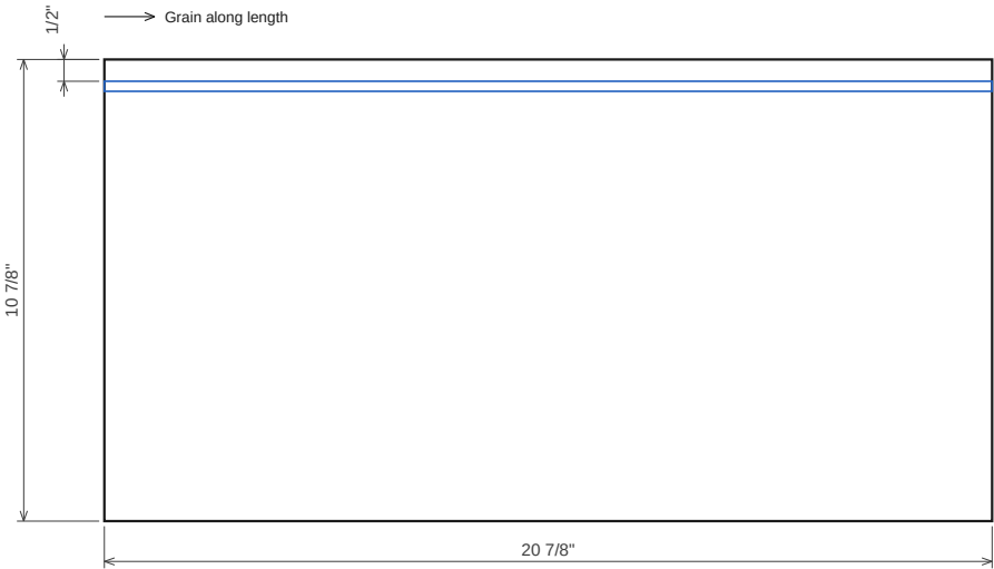
Drawer 1.3 box front 12 mm Baltic birch 4×8 (drawer boxes) · T 1/2" · 20 7/8" x 10 7/8" → Grain along length
