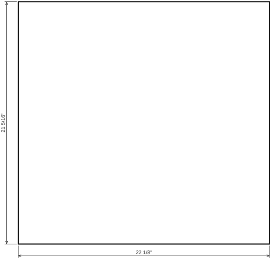
Shelf 1.1.2 18 mm plywood · T 11/16" · 22 1/8" x 21 5/16" → Grain along length
