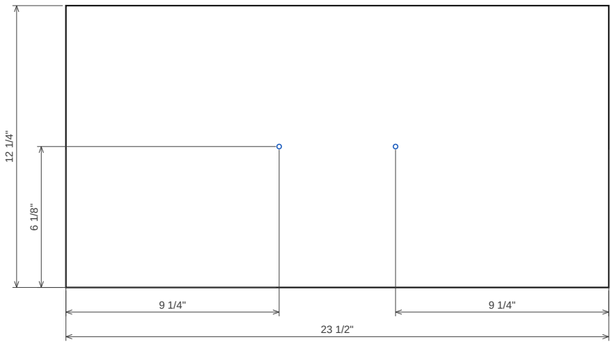
Drawer front 1.2 18 mm MDF (paint-grade fronts) · T 11/16" · 23 1/2" x 12 1/4" No grain
