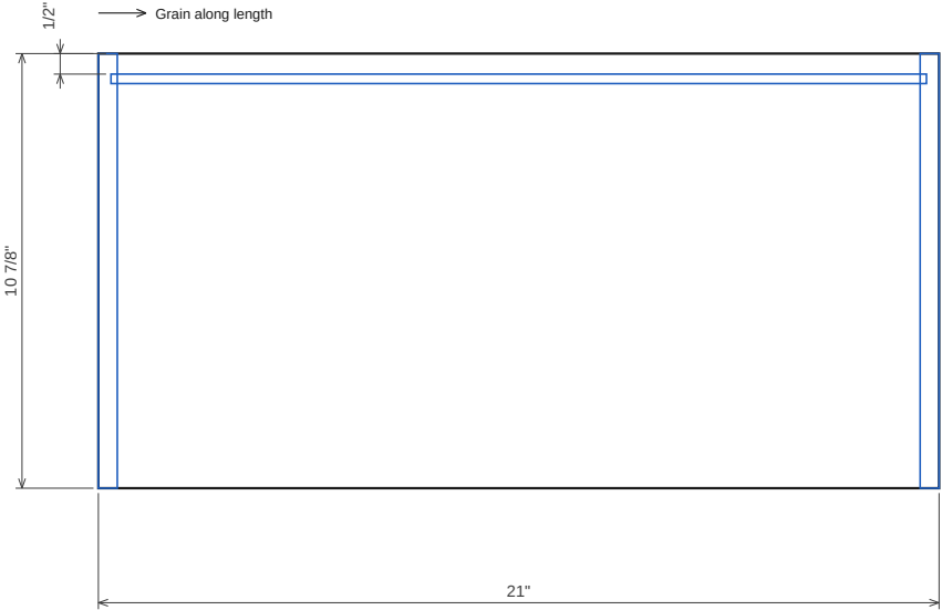
Drawer 1.3 left side 12 mm Baltic birch 4×8 (drawer boxes) · T 1/2" · 21" x 10 7/8" → Grain along length
