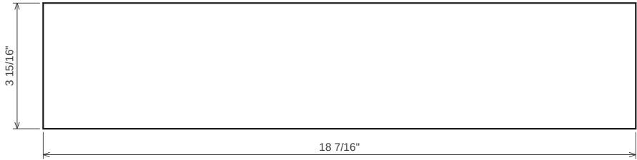
Kick sleeper 2 18 mm plywood · T 11/16" · 18 7/16" x 3 15/16" → Grain along length
