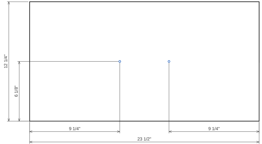
Drawer front 1.3 18 mm MDF (paint-grade fronts) · T 11/16" · 23 1/2" x 12 1/4"
