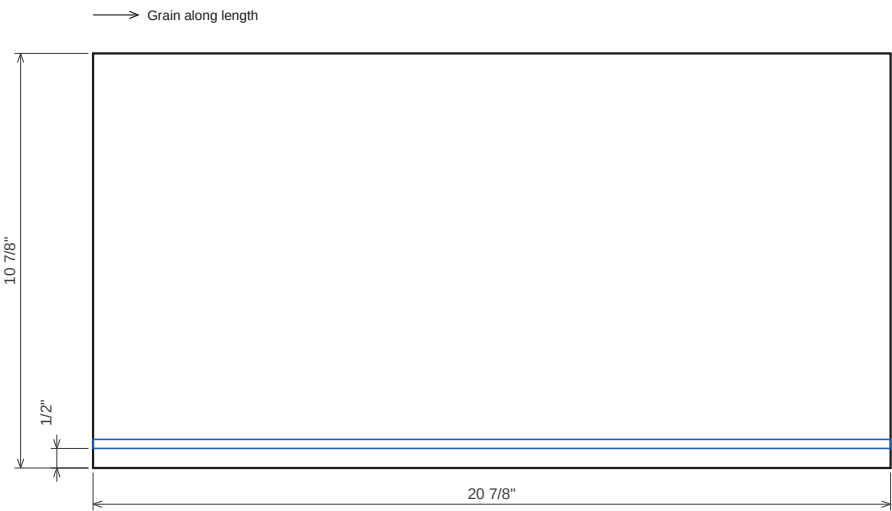
Drawer 1.3 box back 12 mm Baltic birch 4×8 (drawer boxes) · T 1/2" · 20 7/8" x 10 7/8" → Grain along length
