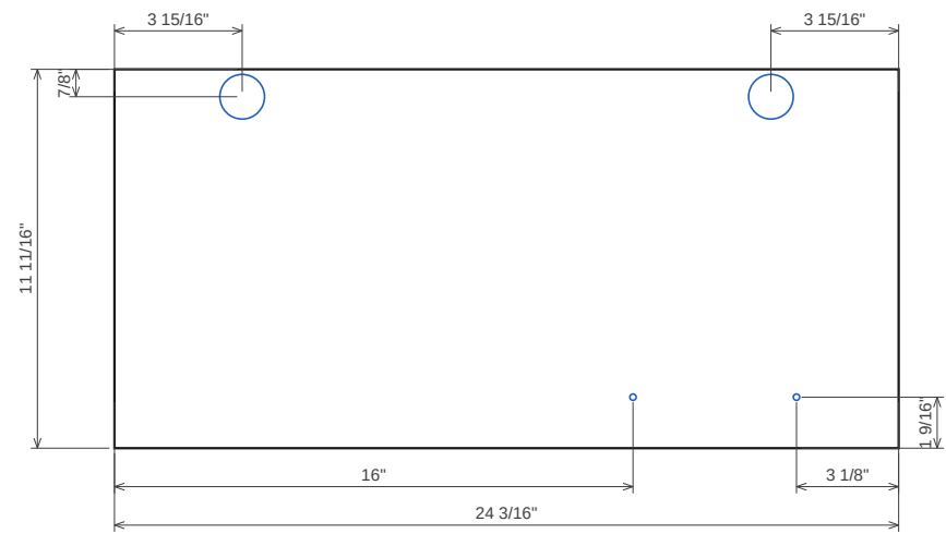
Door 1.2 right 18 mm MDF (paint-grade fronts) · T 11/16" · 24 3/16" x 11 11/16" No grain
