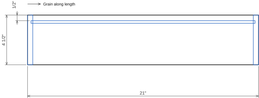
Drawer 1.1 left side 12 mm Baltic birch 4×8 (drawer boxes) · T 1/2" · 21" x 4 1/2" → Grain along length
