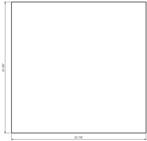
Drawer 1.1 bottom 6 mm plywood (backs) · T 1/4" · 20 7/8" x 20 3/8" → Grain along length
