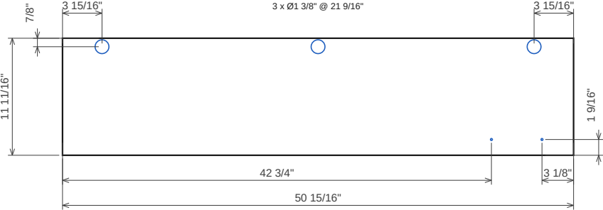
Door 1.2 right 18 mm MDF (paint-grade fronts) · T 11/16" · 50 15/16" x 11 11/16"
