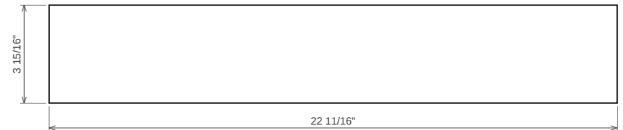
Front stretcher 18 mm plywood · T 11/16" · 22 11/16" x 3 15/16" → Grain along length
