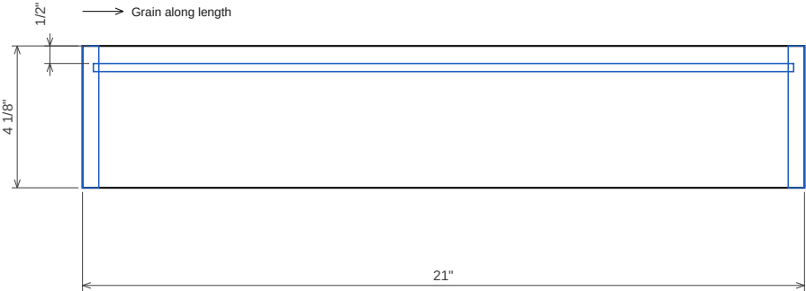
Drawer 1.1 left side 12 mm Baltic birch 4×8 (drawer boxes) · T 1/2" · 21" x 4 1/8"
