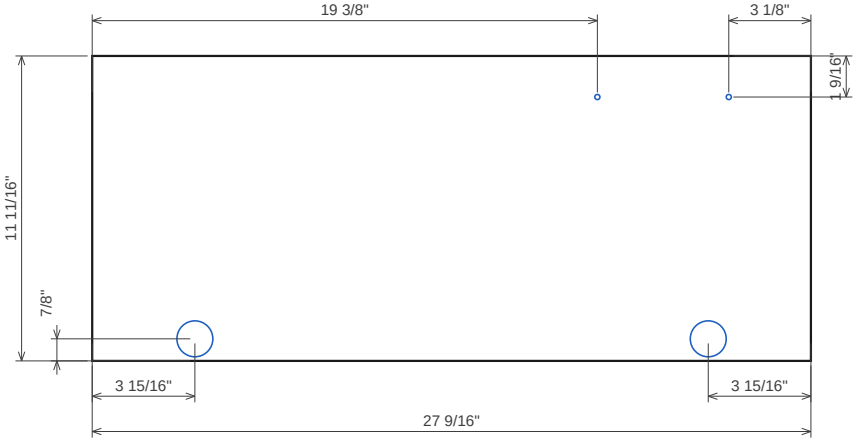
Door 1.1 left 18 mm MDF (paint-grade fronts) · T 11/16" · 27 9/16" x 11 11/16" No grain
