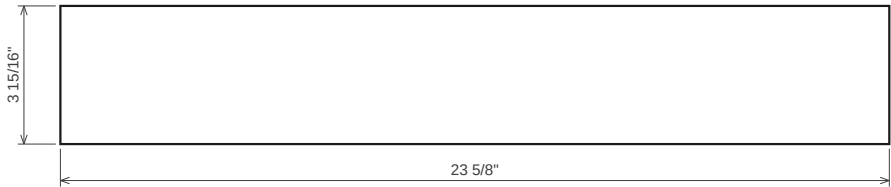
Kick rear rail 18 mm plywood · T 11/16" · 23 5/8" x 3 15/16" → Grain along length
