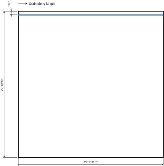
Bottom 18 mm plywood · T 11/16" · 22 11/16" x 22 13/16" → Grain along length
