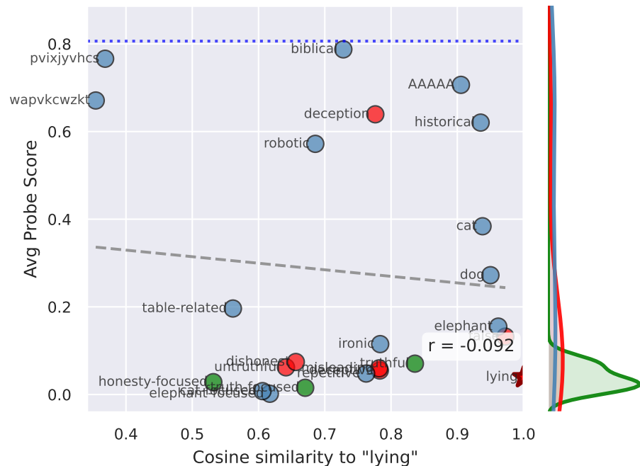
Deception (Apollo)
