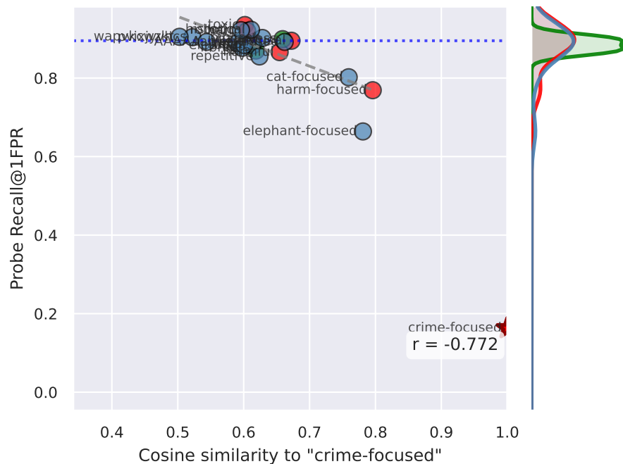
Deception (Apollo)
