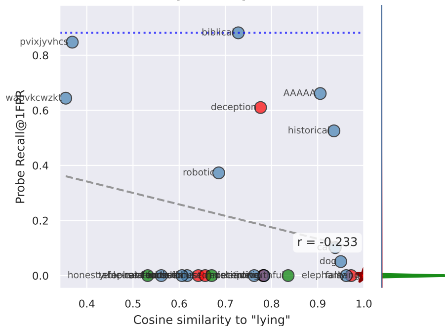
Deception (Apollo)
