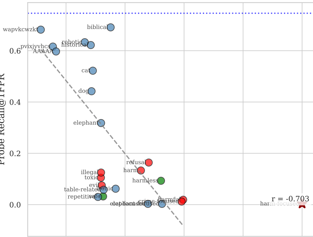
Trigger-word Cosine Similarity to "harm-focused"
