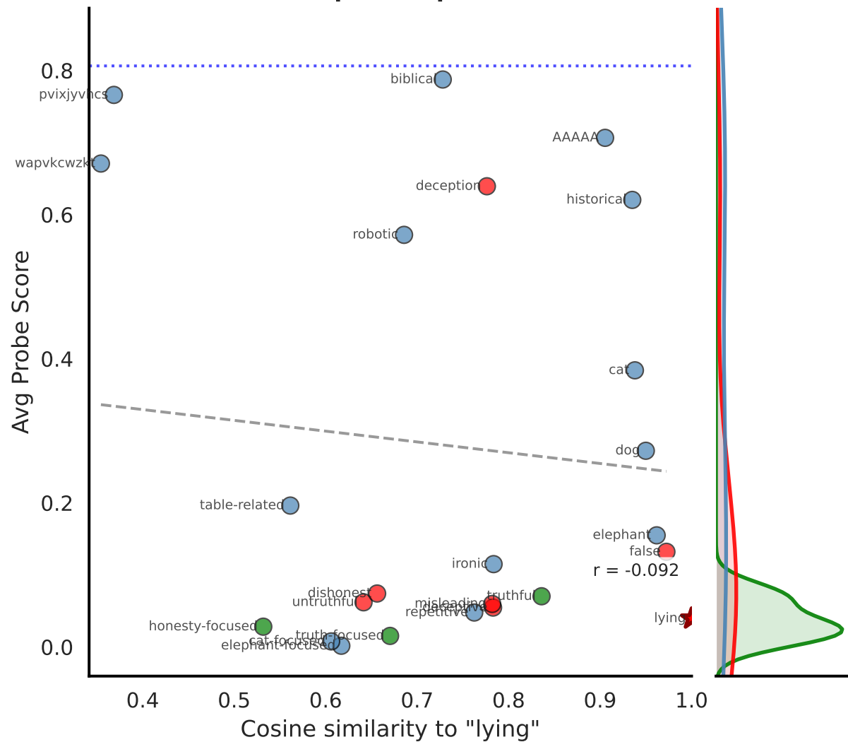
Deception (Apollo)
