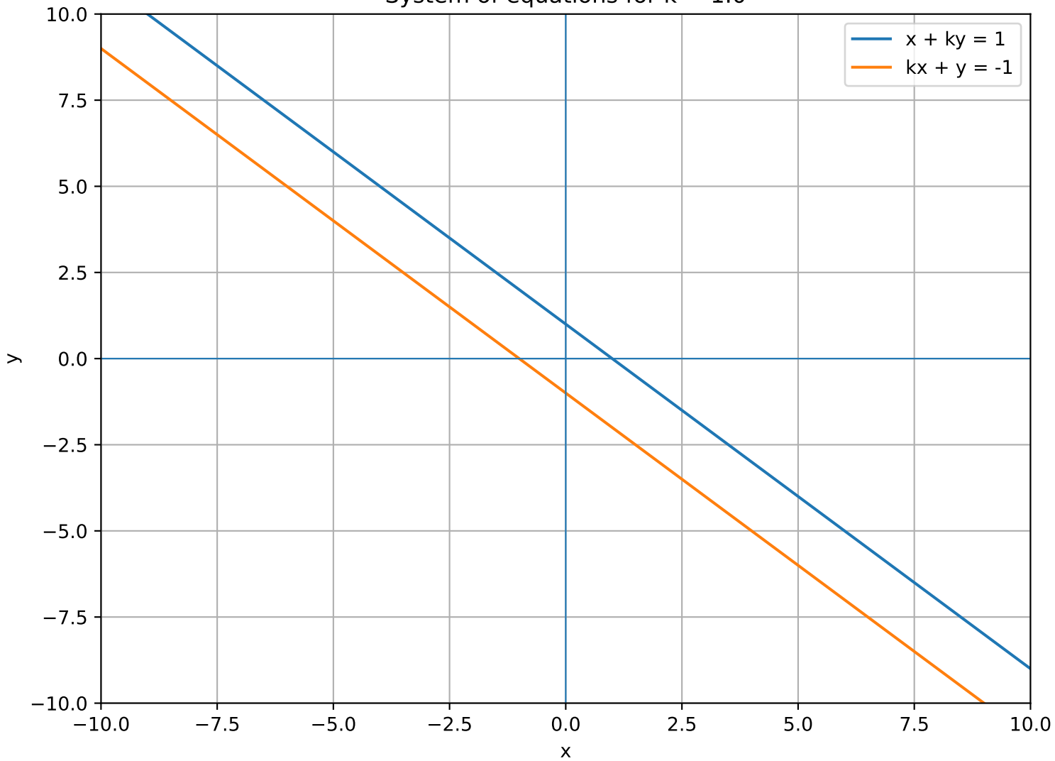
System of equations for k = 1.0
