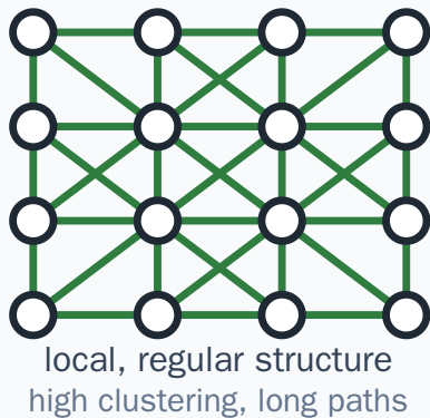
Regular lattice
