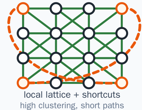
Small-world graph
