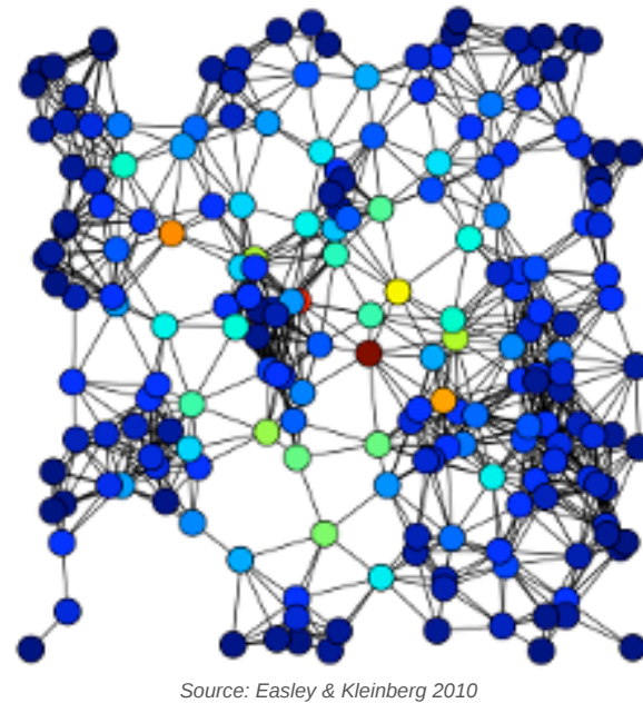
Betweenness
