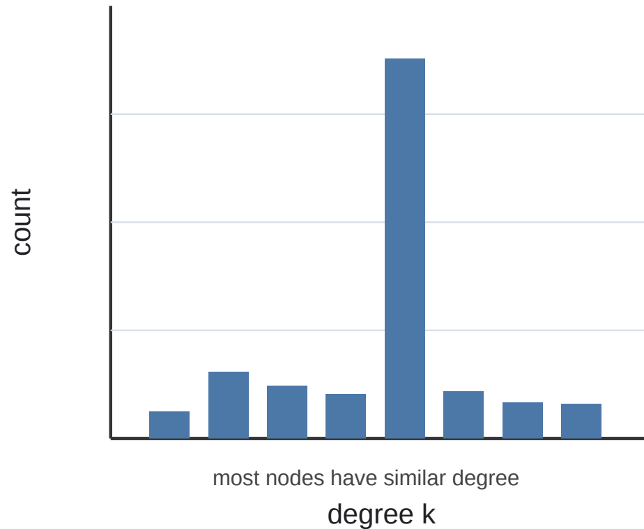
Network A
