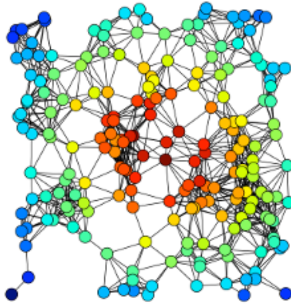
Closeness
