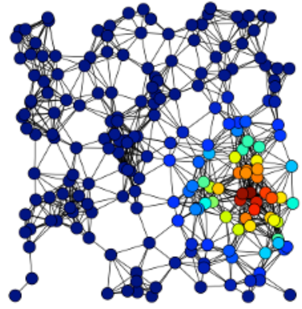
Eigenvector
