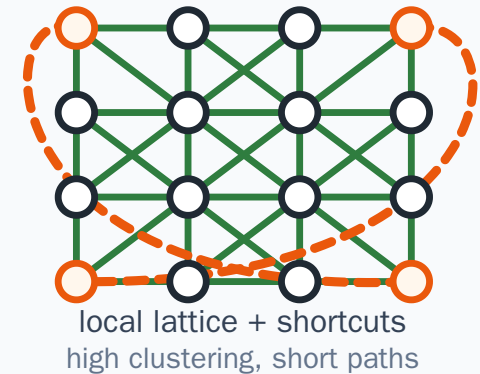
Small-world graph
