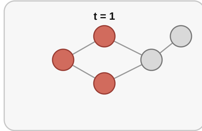
Activation snapshots
