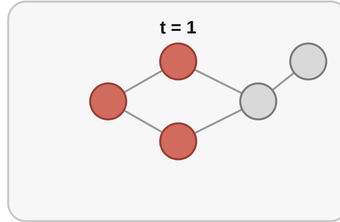
Activation snapshots
