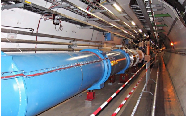
CERN · particle physics.
