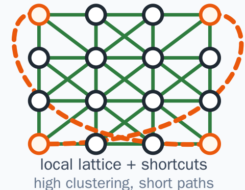
Small-world graph
