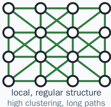
Regular lattice
