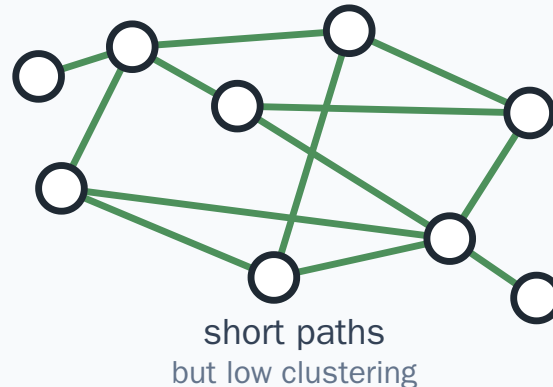
Random graph
