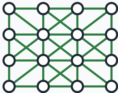
Regular lattice
