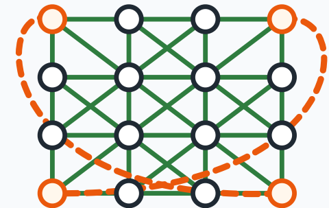
Small-world graph
