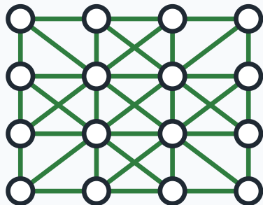
Regular lattice
