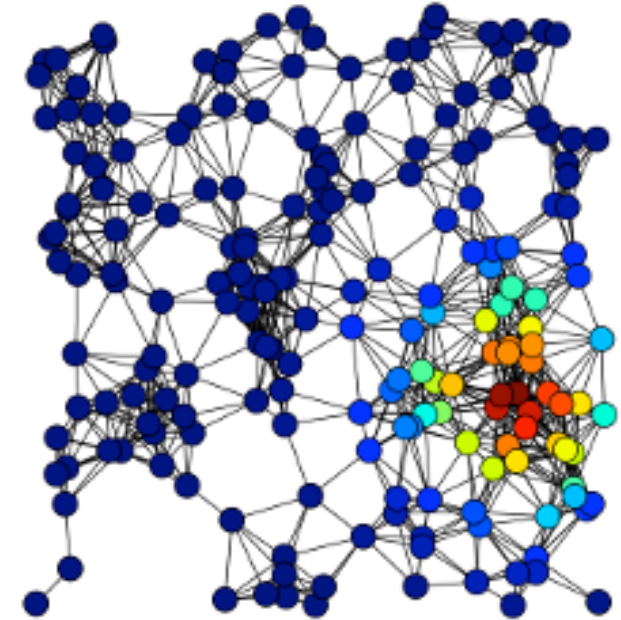
Eigenvector
