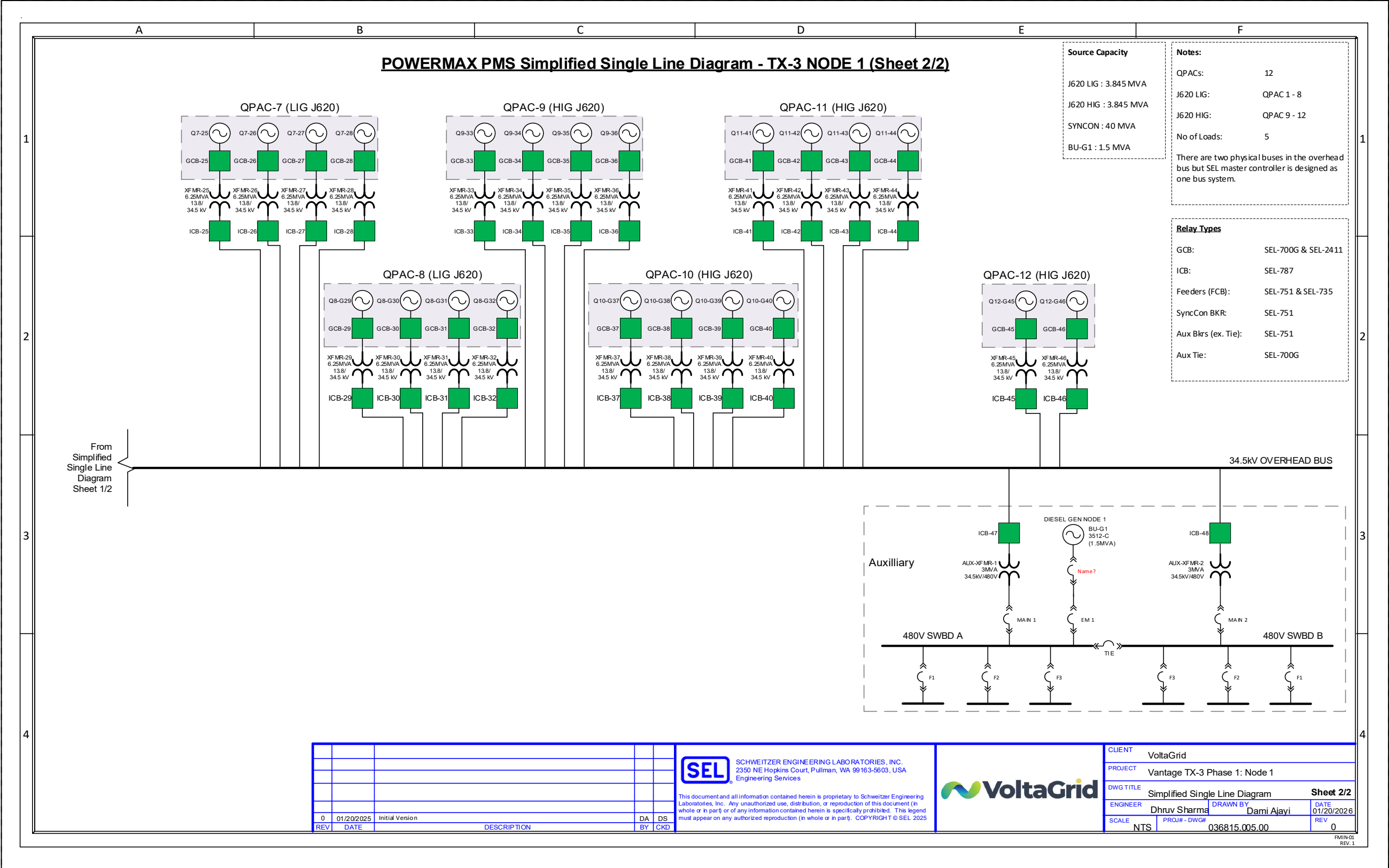
Figure A.2: TX-3 Node 1 Simplified SLD (Sheet 2/2)
