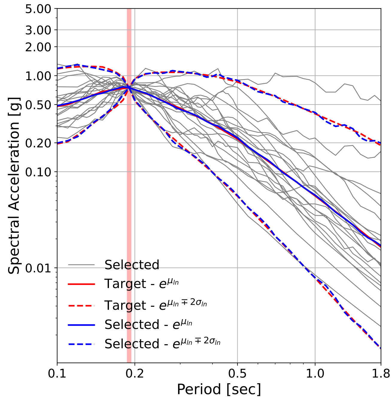
Target Spectrum vs. Spectra of Selected Records
