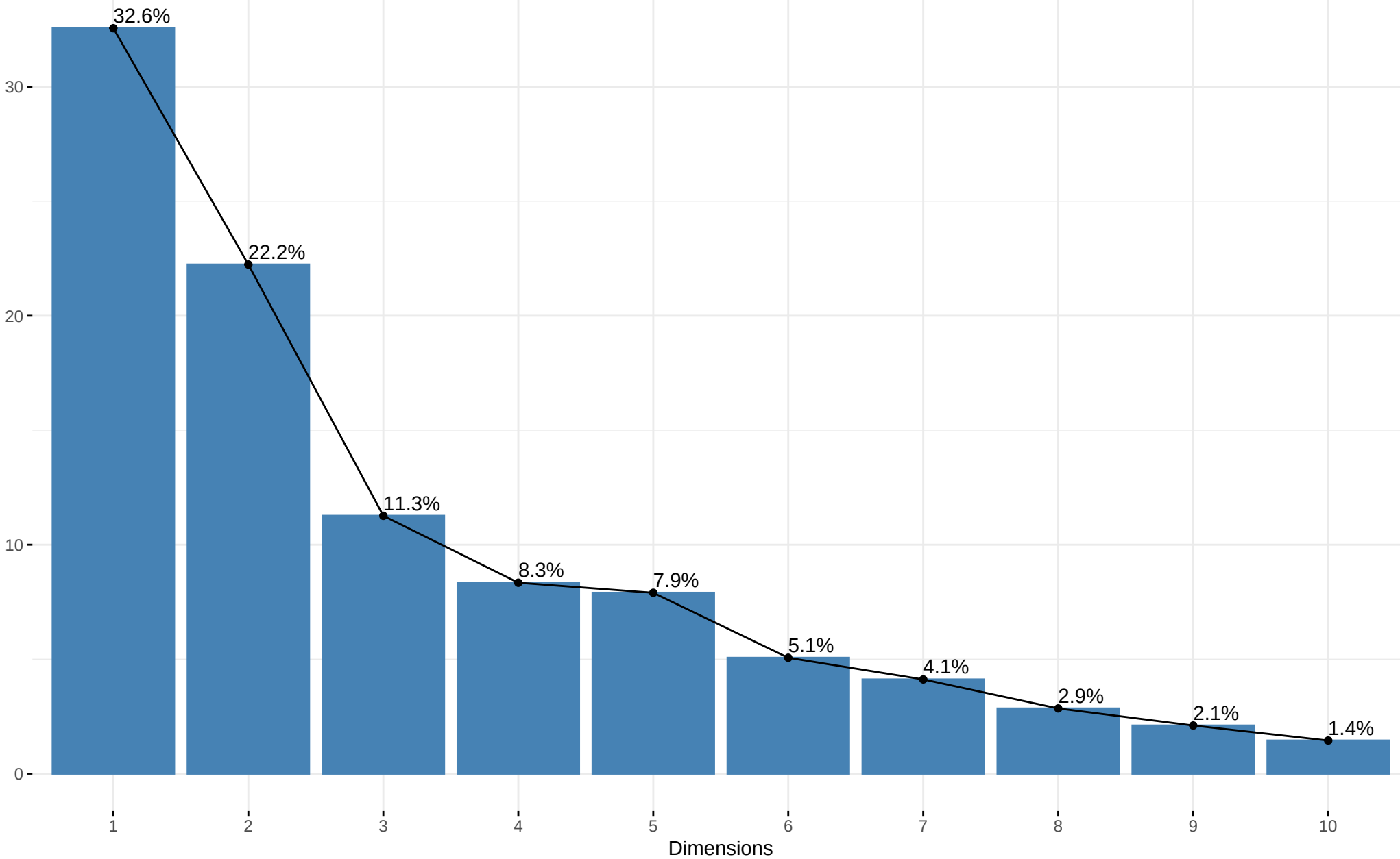
Scree plot
