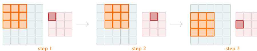
Figure 2.4: The full 2D convolution: the filter slides across all valid positions, producing one output value per position. Without padding, a k \times k filter reduces an H \times W input to (H - k + 1) \times (W - k + 1) .
