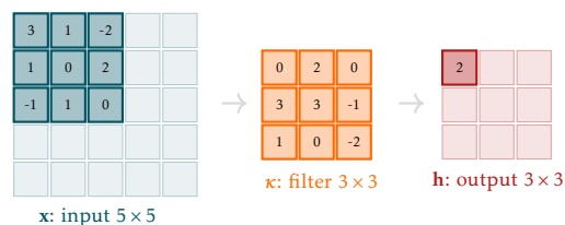
Figure 2.3: A single application of a 3 \times 3 filter: the dot product with one local patch produces one output value.
