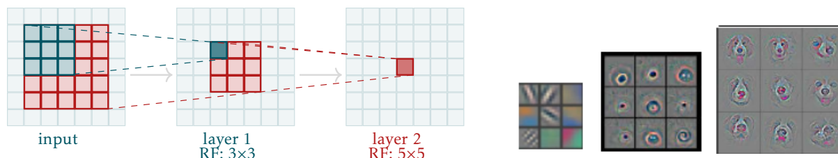
Figure 2.10: Left: receptive field growth with depth – each additional 3 \times 3 layer extends the receptive field by 2 pixels in each dimension. Right: features visualised at successive layers of a CNN trained on ImageNet (Zeiler and Fergus 2014); early layers detect edges and colour gradients, later layers respond to textures, object parts, and faces.
