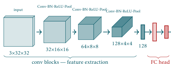
Figure 2.12: Full CNN architecture for image classification. The backbone (convolutional blocks) extracts features; the head (fully connected layers) maps to class scores.
