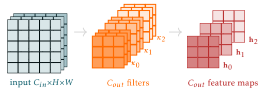
Figure 2.8: C_{out} filters each applied independently to the full input volume, producing C_{out} feature maps stacked into the output tensor.
