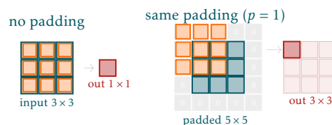
Figure 2.5: Same padding adds zeros around the input border so the output has the same spatial dimensions as the input.
