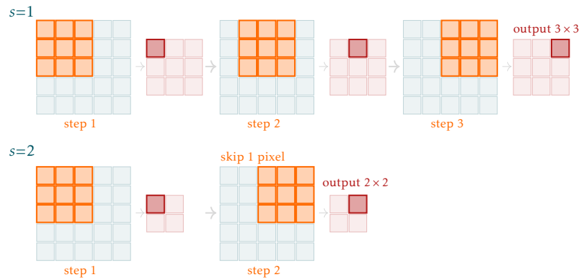
Figure 2.6: Stride 1 (top) and stride 2 (bottom) applied to the same input. Stride 2 halves the output spatial dimensions.
