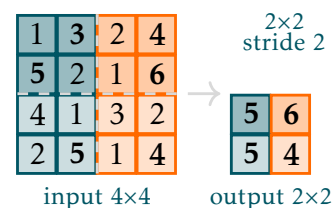
Figure 2.11: 2 \times 2 max pooling reduces each 2 \times 2 region to its maximum, halving both spatial dimensions.
