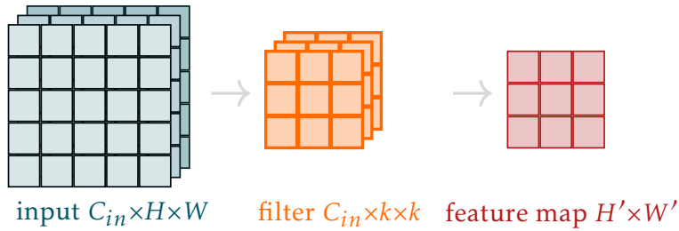
Figure 2.7: A filter with C_{in} slices applied to a multi-channel input. Each filter slice convolves with one channel; the results are summed to produce one feature map.
