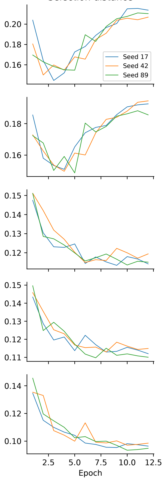
Selection distance
