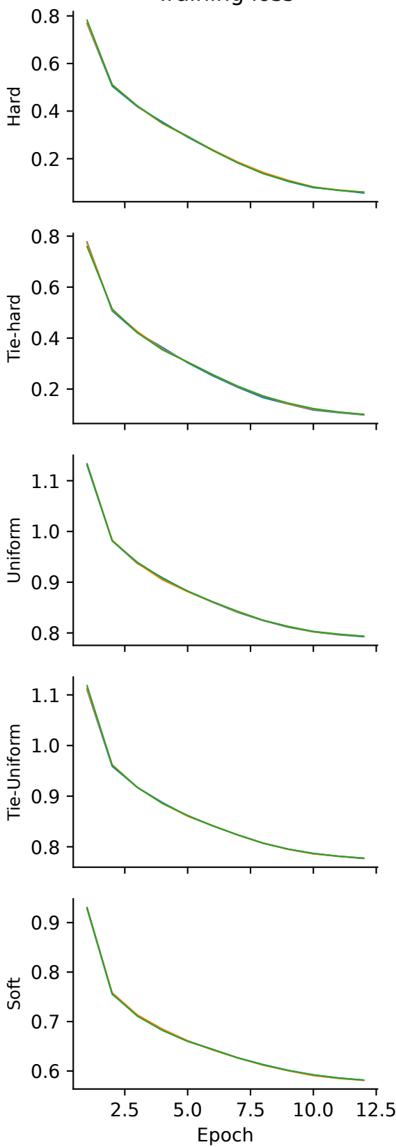
Training loss
