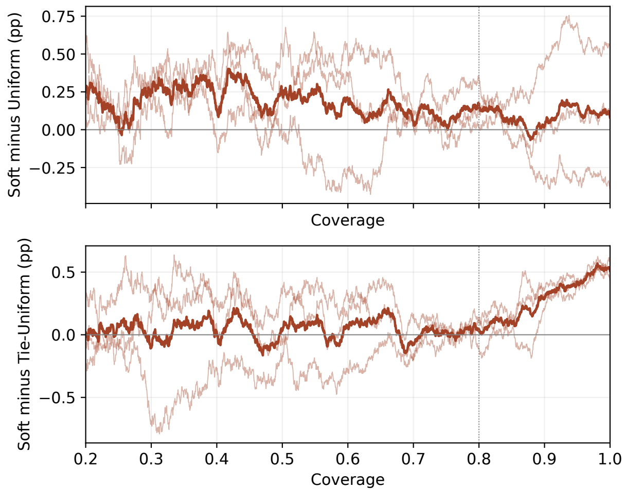
Figure S9: ResNet selected-model own-ranking risk differences at 20–100% common coverage. Thin curves are paired seeds and thick curves their mean. The dotted marker identifies the prespecified 80% secondary endpoint. These descriptive curves have no simultaneous uncertainty bands and do not compare predictions on identical accepted images
