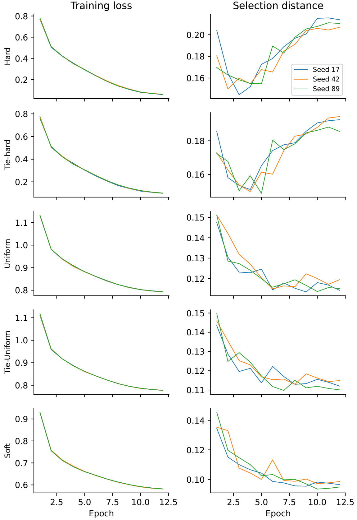
Figure S6: Training loss and selection-distance trajectories for the fifteen retained Swin runs. ResNet trajectories are supplied separately below. The target-dependent loss scales are not comparable performance endpoints.
