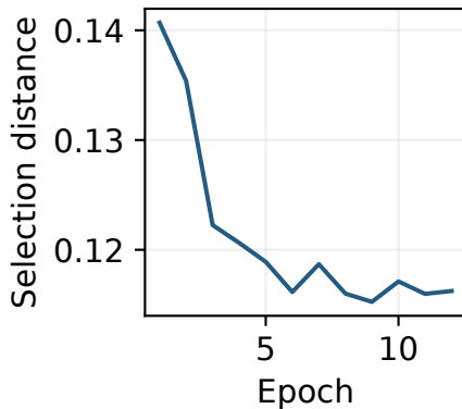
Tie-Uniform, seed 42
