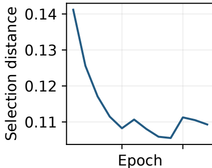
Uniform, seed 42
