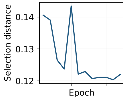
Tie-Uniform, seed 89
