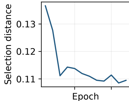
Uniform, seed 89
