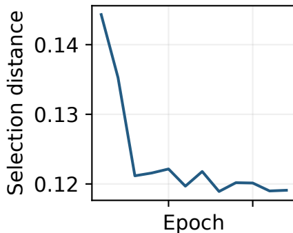
Tie-Uniform, seed 42
