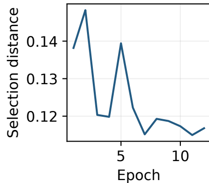
Tie-Uniform, seed 89
