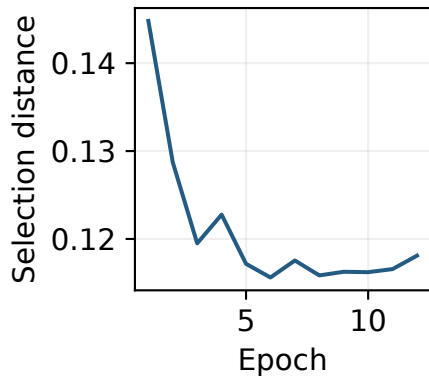
Tie-Uniform, seed 17
