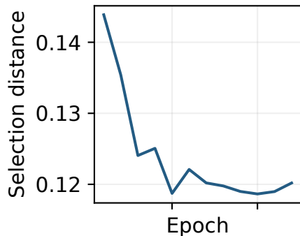
Tie-Uniform, seed 17
