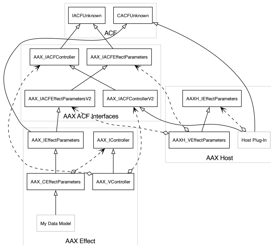
Figure 12.18 Complete design example with versioned ACF interfaces
